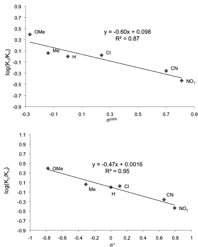
Figure 1. Hammett plots.
